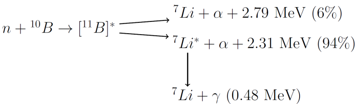
Figure 1: Boron capture reaction. Source: the authors.
