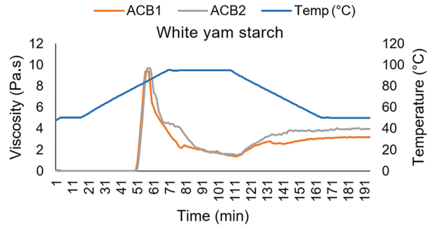
Figure 4 – Viscoamylogram of white yam starch (ACB) obtained by Rapid Visco Analyzer (RVA), in duplicate. Temp = temperature.
