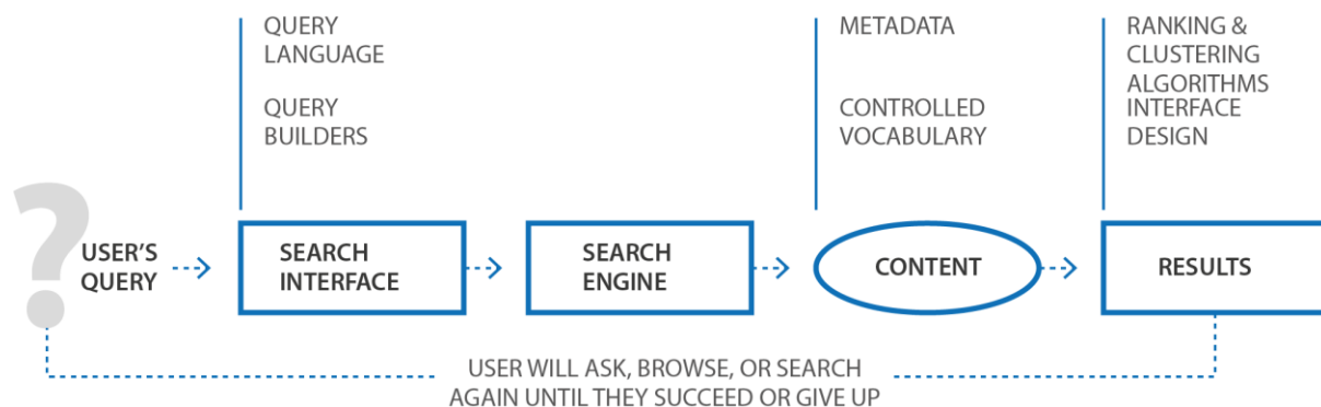
Figure 1. Search System
