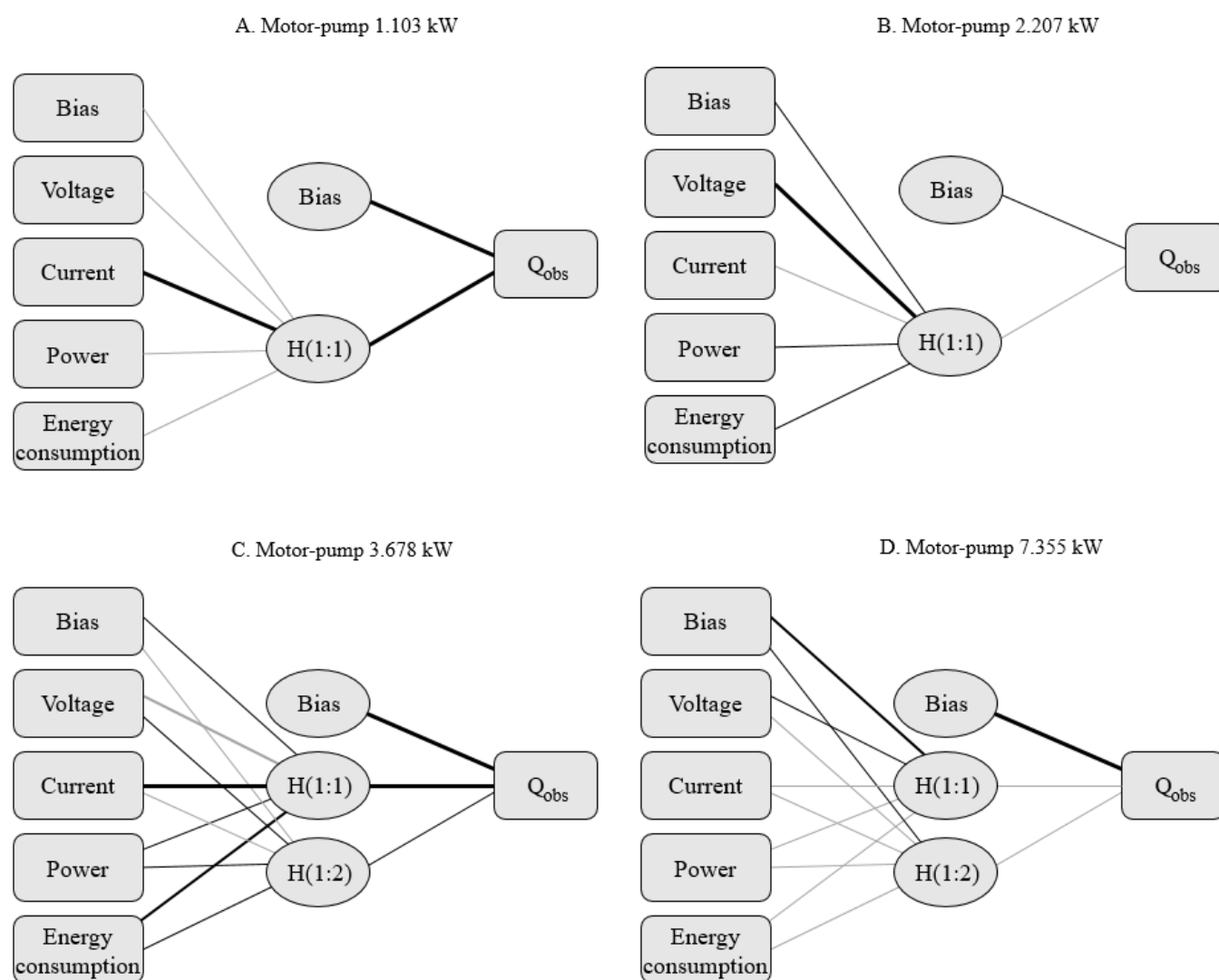
Figure 1. Artificial neural network architectures for the input variables in motor-pump sets of 1.103 kW (A), 2.207 kW (B), 3.678 kW (C), and 7.355 kW (D)
