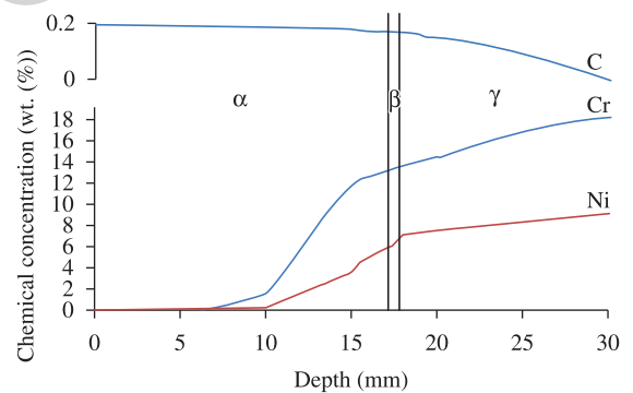
Figure 3. The chemical profile of chromium, nickel and carbon atoms in FGS formed at remelting stage.
