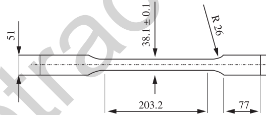
Figure 2. Dimension of tensile composite specimen (mm).
