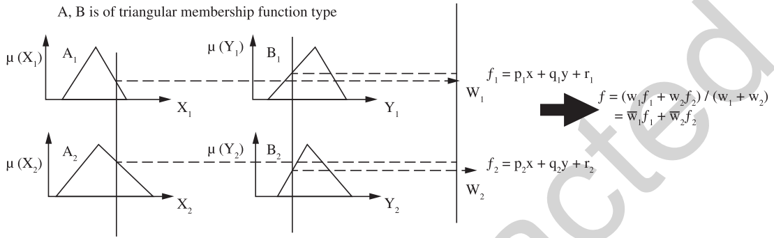
Figure 6. The reasoning scheme of ANFIS 49 .
