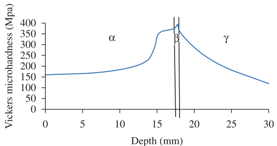
Figure 1. Vickers microhardness profile of the produced FGS.
