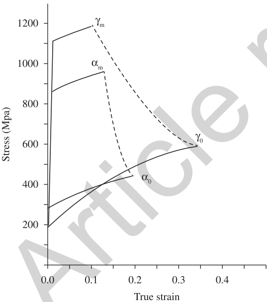
Figure 5. True stress-strain curves of \gamma_0 , \alpha_0 , \gamma_m and \alpha_m layers.
