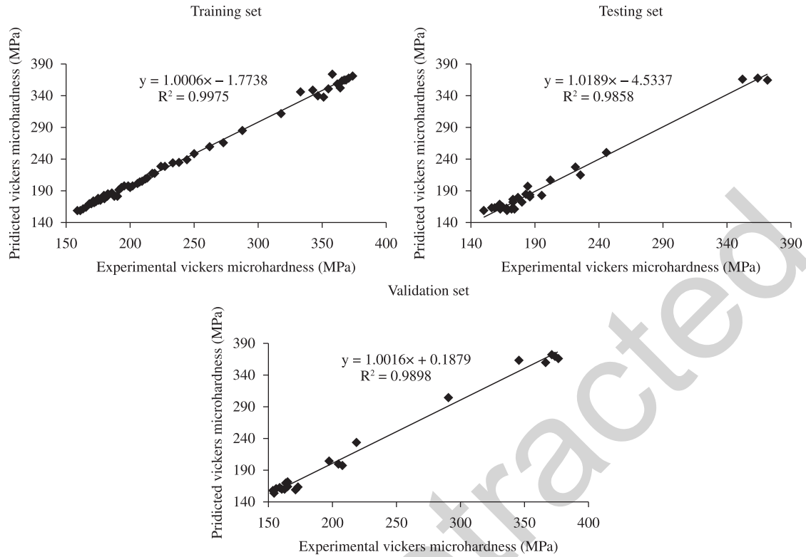
Figure 8. The correlation of the measured and predicted Vickers microhardness values in a) training; b) testing; and c) validation sets for ANFIS-I model.
