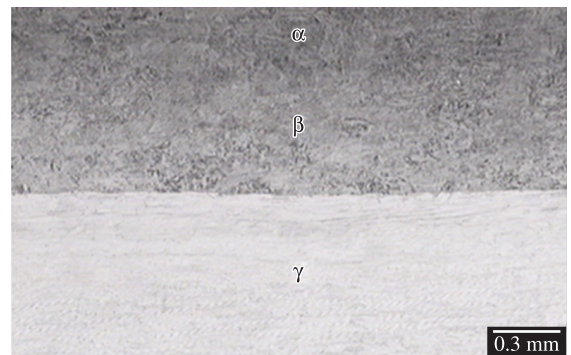
Figure 4. Microstructure of the produced FGS.
