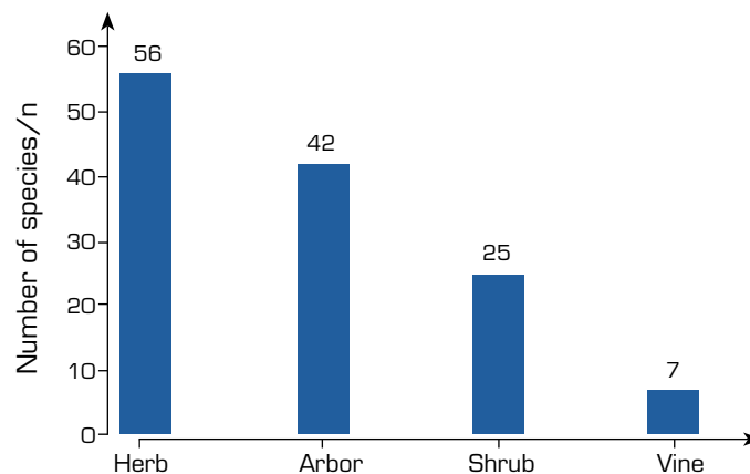
Figure 3. Plant species statistics.
