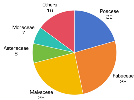
Figure 4. Statistical results of the species families.
