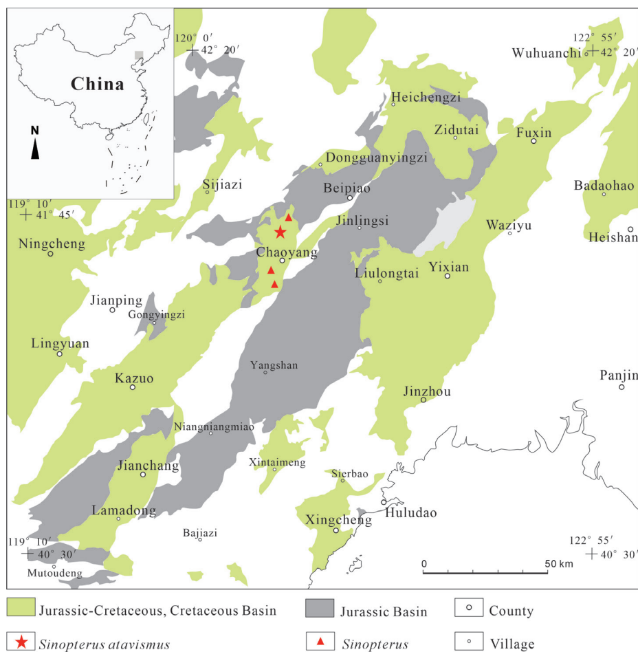
Figure 1. The distribution of fossils of Sinopterus and a sketched geological map of western Liaoning.
